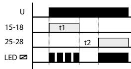
CRM-2T/24-480V
