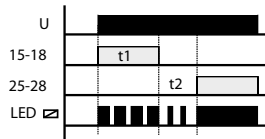
CRM-2T/UNI, CRM-2T/230V
